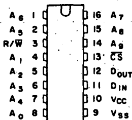
PIN NAMES
